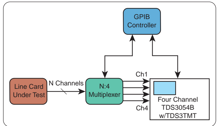
► Figure 3. System design for maximized throughput using TDS3000B multi-channel testing.
